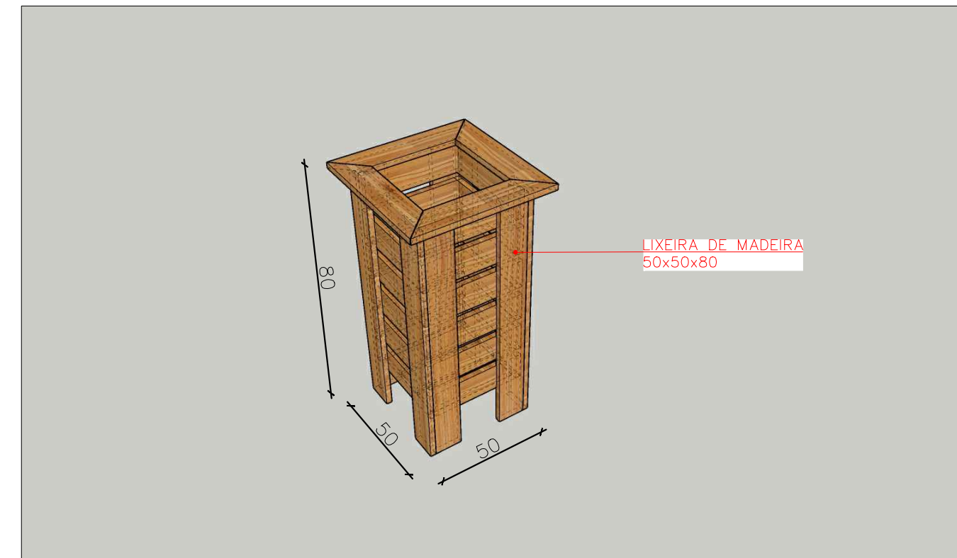
LIXEIRA 50X50X80
